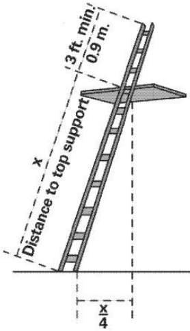
Figure D-1 -- Portable Ladder Set-up
