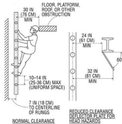
Figure D-5 -- Fixed Ladder Clearances
